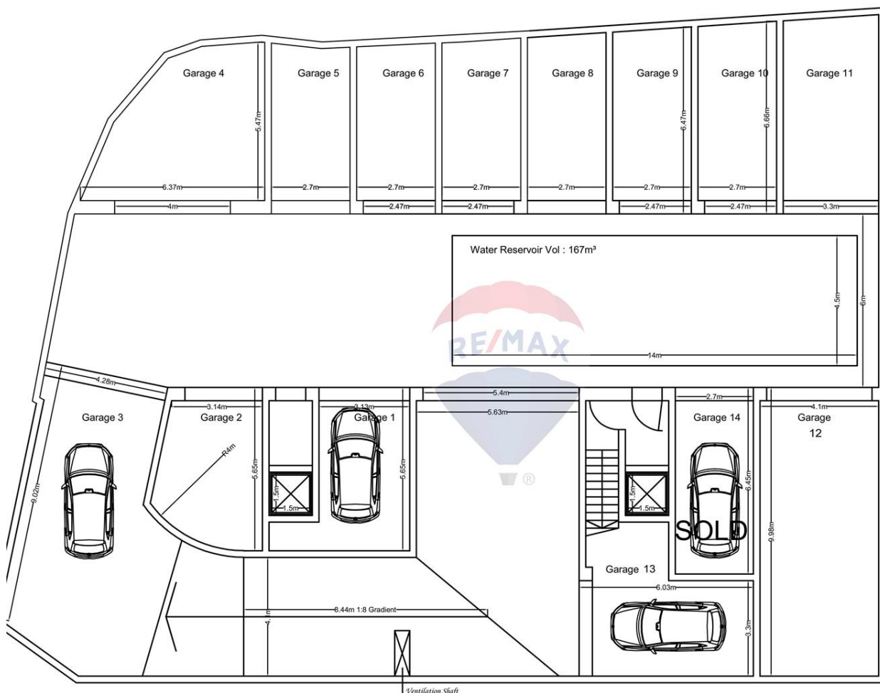
Proposed Basement -2
