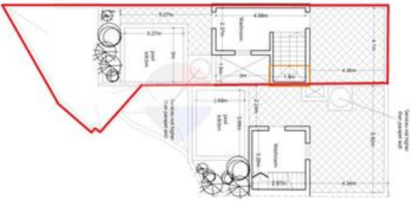
Proposed revised floor plan
