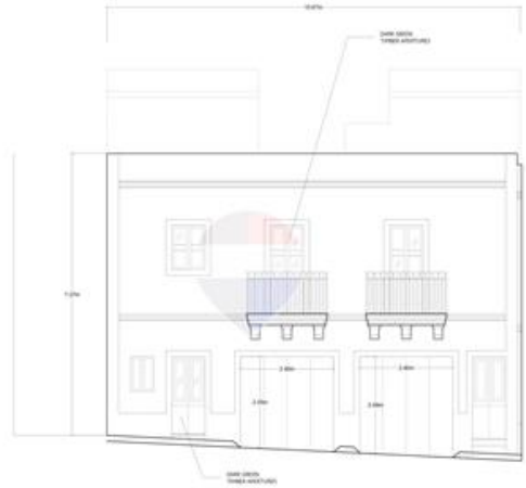
Proposed Front Elevation Scale 1:50 Clean copy
