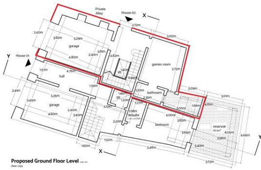
Proposed Ground Floor Level clean copy
