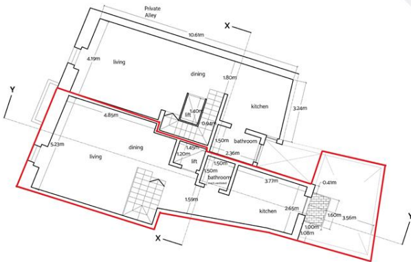
Proposed Second Floor Level clean copy
