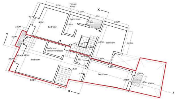
Proposed First Floor Level clean copy
