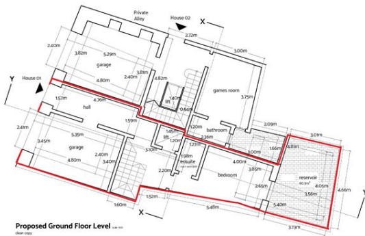
Proposed Ground Floor Level clean copy
