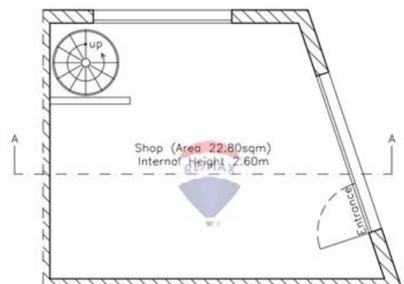
Floor Plan Existing Scale 1:50
