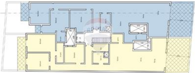
PENTHOUSE LEVEL
