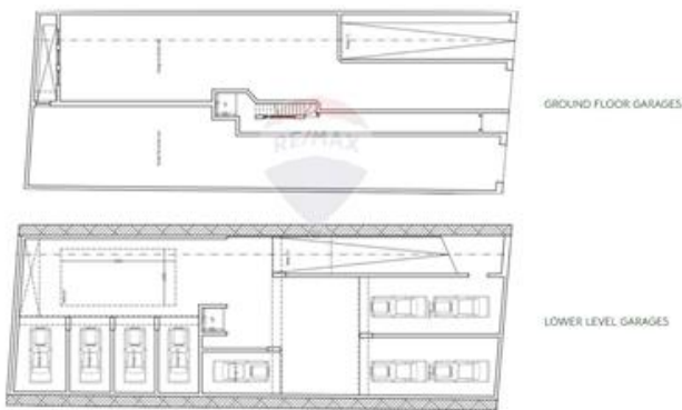
GARAGES
