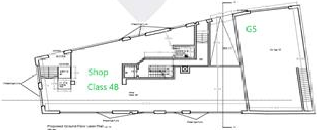
Proposed Basement Floor Level Plan
