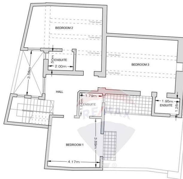
PROPOSED FIRST FLOOR - Clean Copy Scale 1:100
