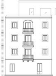
BACK ELEVATION ON THE JOHN D'AMICO STREET 100
