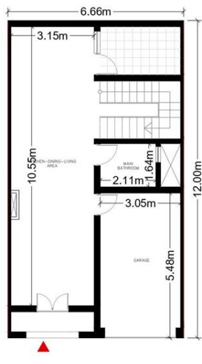
GROUND FLOOR scale 1 : 100
