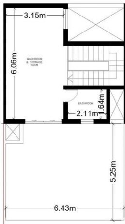
SECOND FLOOR scale 1 : 100
